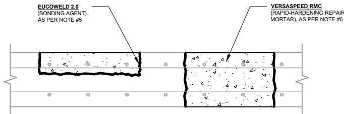
COMPLETED REPAIR
