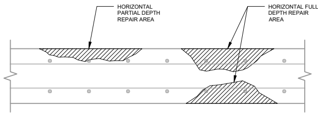
EXISTING CONDITION
