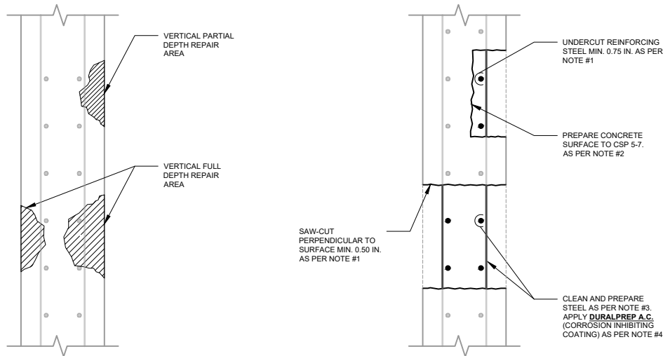
EXISTING CONDITION
