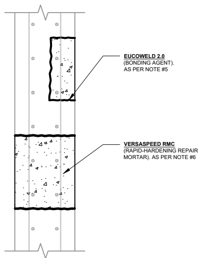
COMPLETED REPAIR
